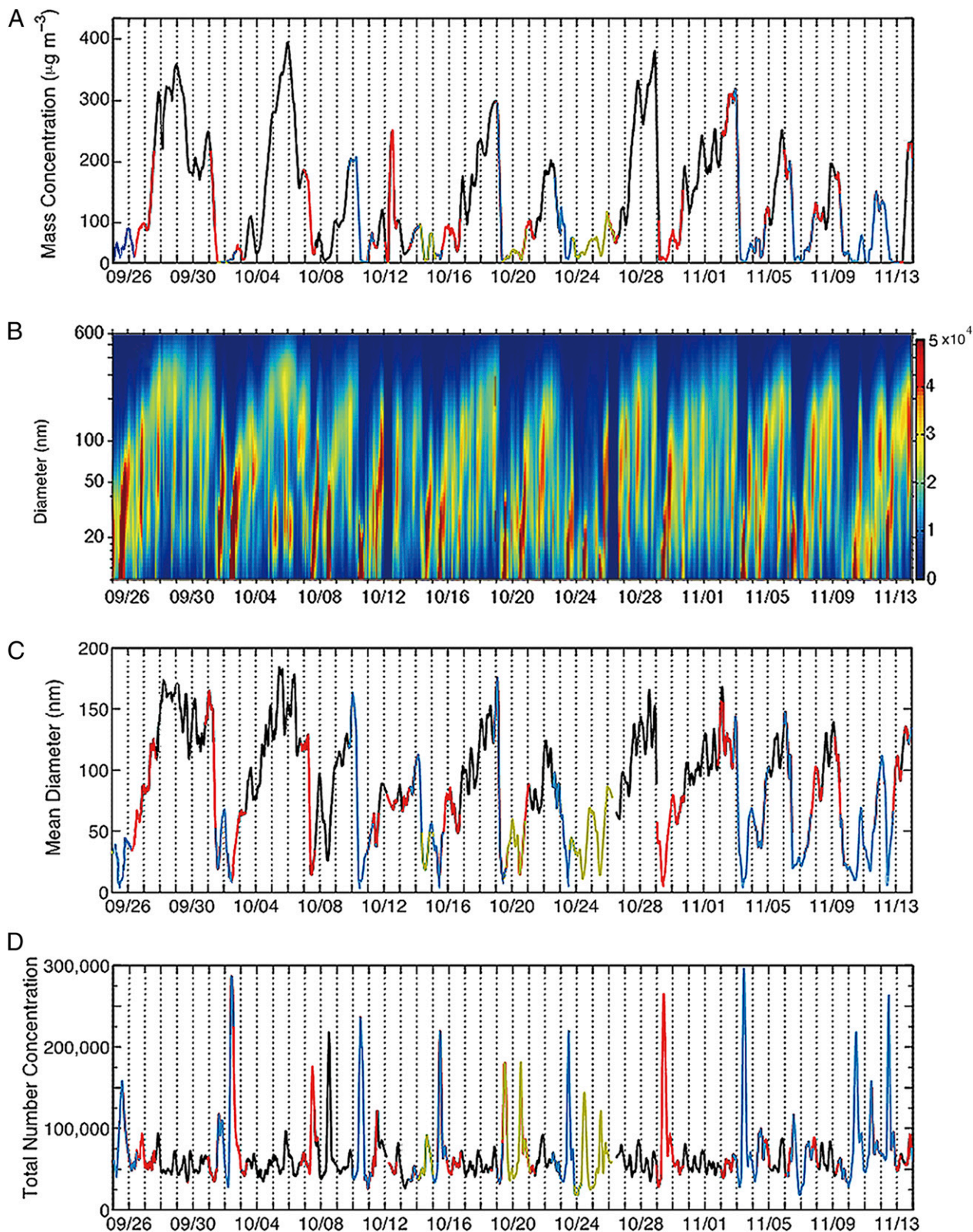
Fig. 1. Periodic PM_{2.5} cycles in Beijing. Temporal evolutions of PM_{2.5} mass concentration (A), number size distribution (B), mean diameter (C), and total number concentration (D) during the PM_{2.5} events from 25 September through 14 November 2013. The colors in A, C, and D represent the air mass originating from the south (black), northwest (blue and red), and northeast (yellow), similar to those in Fig. S1. The color contour in B denotes the particle number concentration, i.e., dN/d\log D ( cm^{-3} ) on the right vertical axis (where N and D represent the particle number and size, respectively). Each PM_{2.5} cycle includes a clean period in the beginning, a polluted period in the end, and their transition. The dates on the x axis (also the vertical lines) correspond to midnight local time. The mean particle diameter is computed using a log-normal function from each measured size distribution at a given time.
