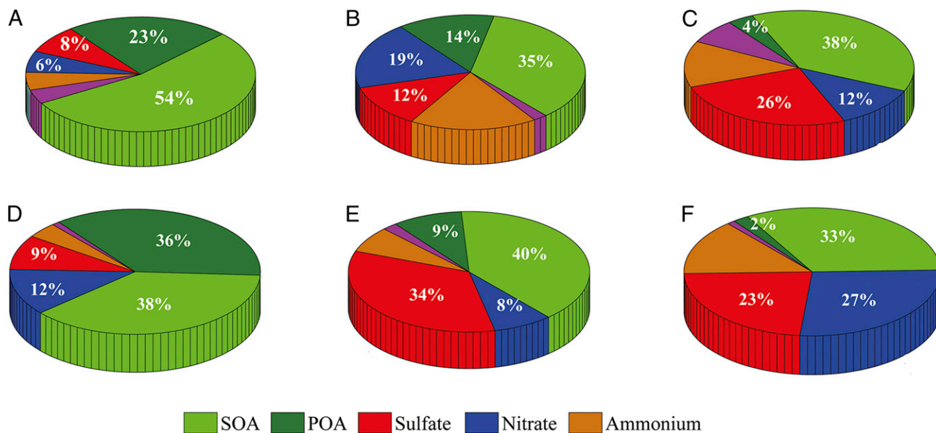
Fig. 3. Particle chemical compositions during the clean, transition, and polluted periods for the 25–29 September and 2–7 October episodes. (A–C) Chemical compositions for 80-nm (A), 100-nm (B), and 240-nm (C) particles measured by the AMS at 1500 h on 25 September, 1200 h on 27 September, and 1800 h on 28 September, respectively. The three particle sizes (i.e., close to the mean size) are selected to represent the dominant features in the chemical composition during the clean, transition, and polluted periods. At the three times, the hourly average PM_{2.5} mass concentrations are 12 \mu g \cdot m^{-3} , 167 \mu g \cdot m^{-3} , and 288 \mu g \cdot m^{-3} , and the particle mean diameters are 25 nm, 96 nm, and 151 nm, respectively. The mass concentrations of primary organic aerosols are 3 \mu g \cdot m^{-3} , 14 \mu g \cdot m^{-3} , and 13 \mu g \cdot m^{-3} corresponding to A, B, and C, respectively, consistently small throughout the episode. (D–F) Chemical compositions for 80-nm (D), 100-nm (E), and 240-nm (F) particles at 1500 h on 2 October, 1200 h on 4 October, and 1200 h on 5 October, respectively. The hourly average PM_{2.5} mass concentrations at the three times are 14 \mu g \cdot m^{-3} , 111 \mu g \cdot m^{-3} , and 312 \mu g \cdot m^{-3} , and the particle mean diameters are 21 nm, 98 nm, and 192 nm, respectively. The numbers for the colors denote the mass concentrations of the aerosol constituents, i.e., light green for secondary organics, dark green for primary organics, blue for nitrate, red for sulfate, yellow for ammonium, and purple for chloride. The ammonium (yellow) mass fractions are 5% (A), 18% (B), 13% (C), 4% (D), 7% (E), and 14% (F), and the chloride (purple) mass fractions are 4% (A), 2% (B), 7% (C), 1% (D), 2% (E), and 1% (F).
